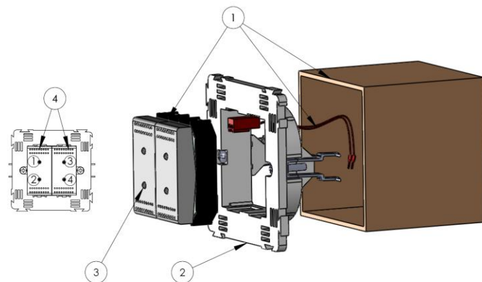
Figure 2 : Connection Bticino® switch SWC04.
